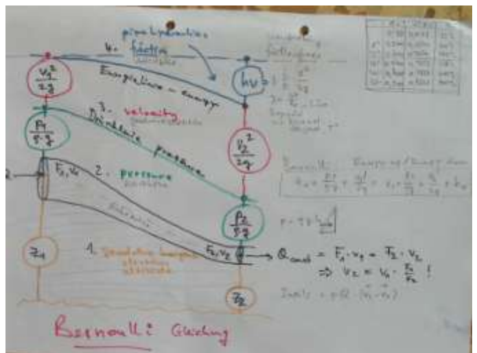
Bernoulli Equation for Net work Analysis of Main pipes with booster stations and pumping station 1. Geodetic height, Pressure, Velocity, Loss of Energy ... Volume constant: A(i) \cdot v(i) .
